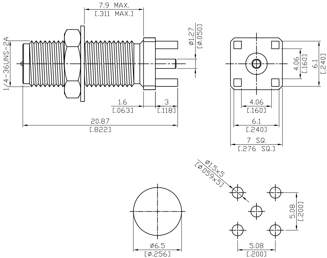
MOUNTING HOLE
