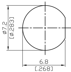
MOUNTING HOLE
