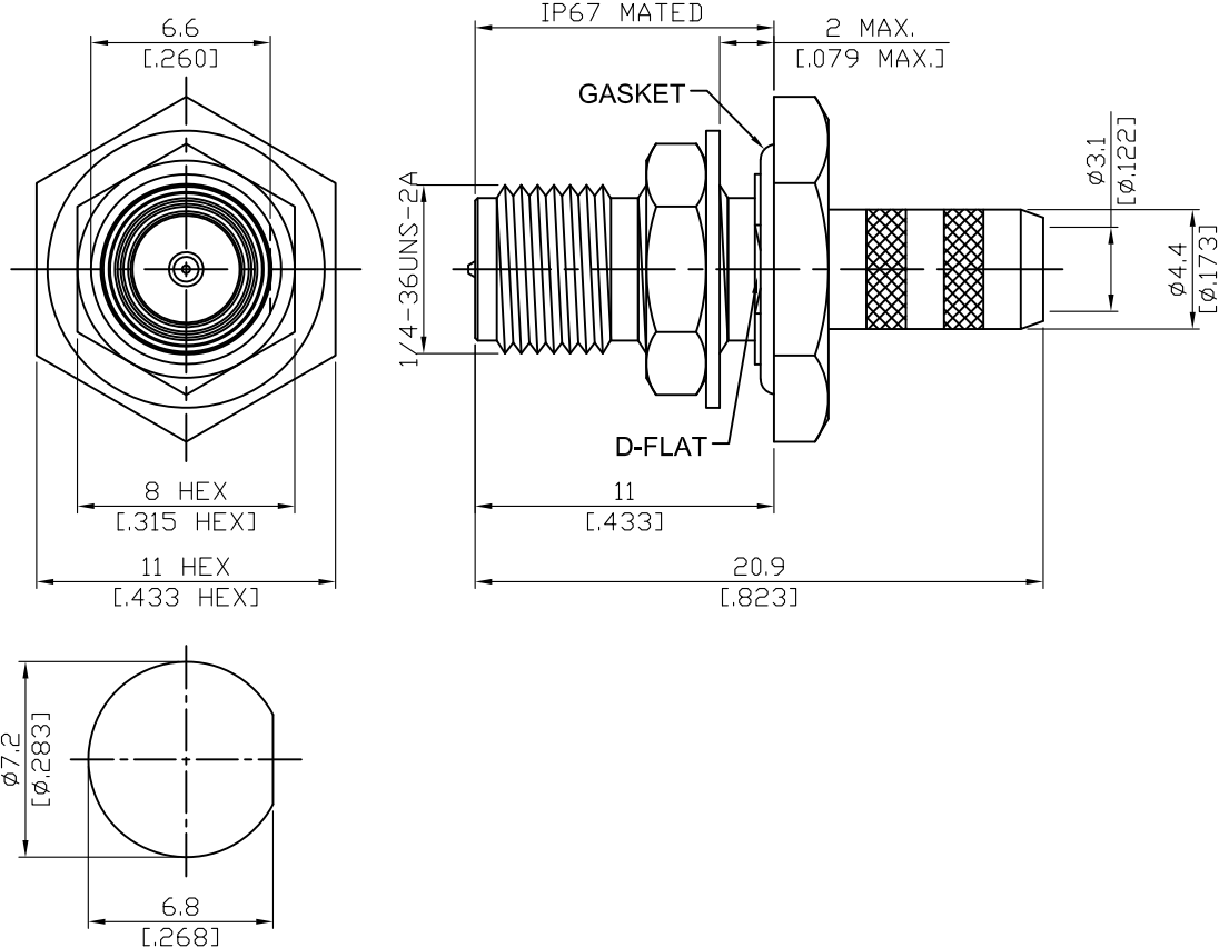
MOUNTING HOLE
