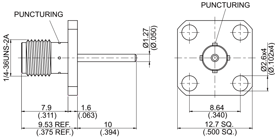
MOUNTING HOLE
