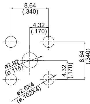
MOUNTING HOLE
