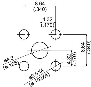
MOUNTING HOLE
