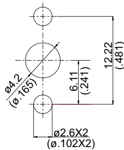
MOUNTING HOLES
