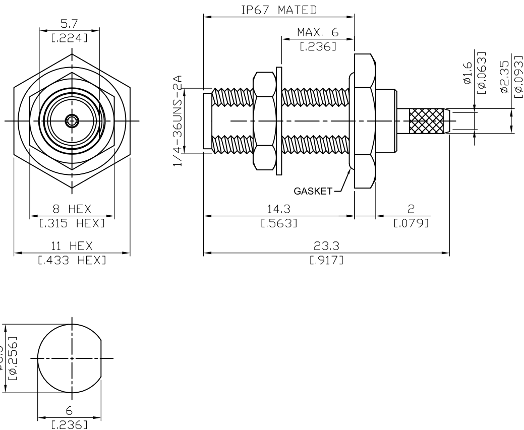
MOUNTING HOLE
