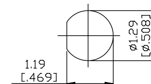
MOUNTING HOLE
