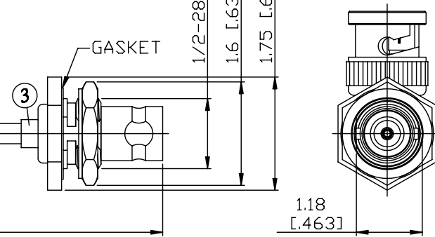
BNC FEMALE FOR BULKHEAD
