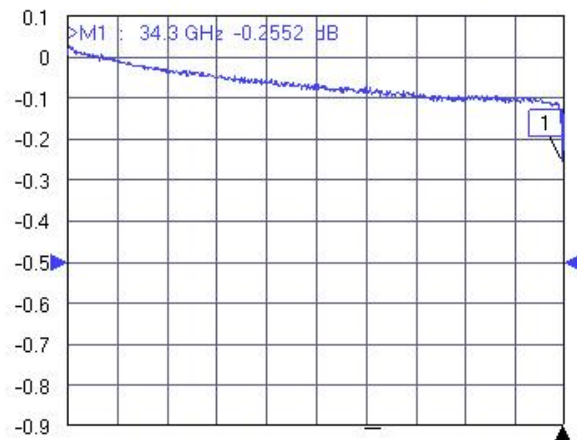
Tr3 S21 Trans LogM RefLvl: -0.5 dB Res: 0.1 dB/Div
