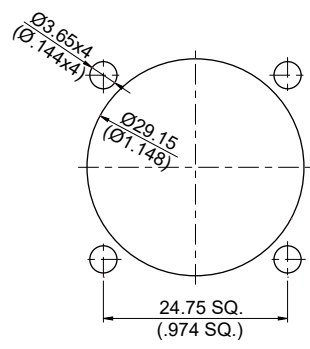
MOUNTING HOLE
